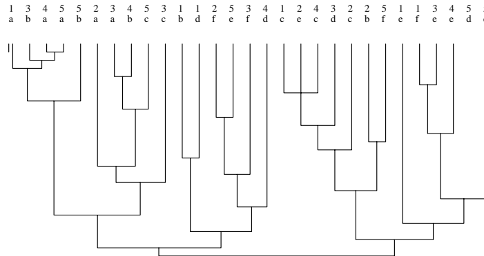
Similarity tree
