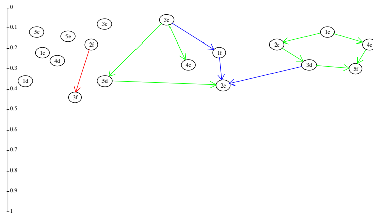
Implicative graph
